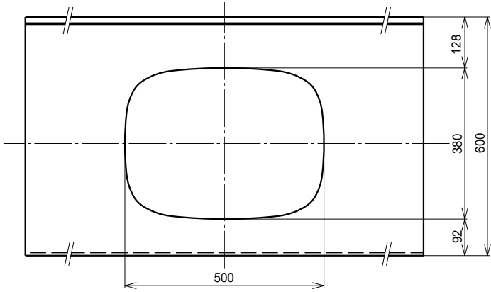
Plane view from bottom
