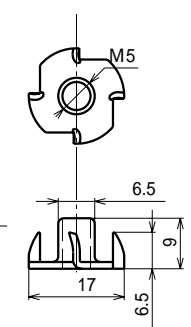
Ratchet nut (M5)
